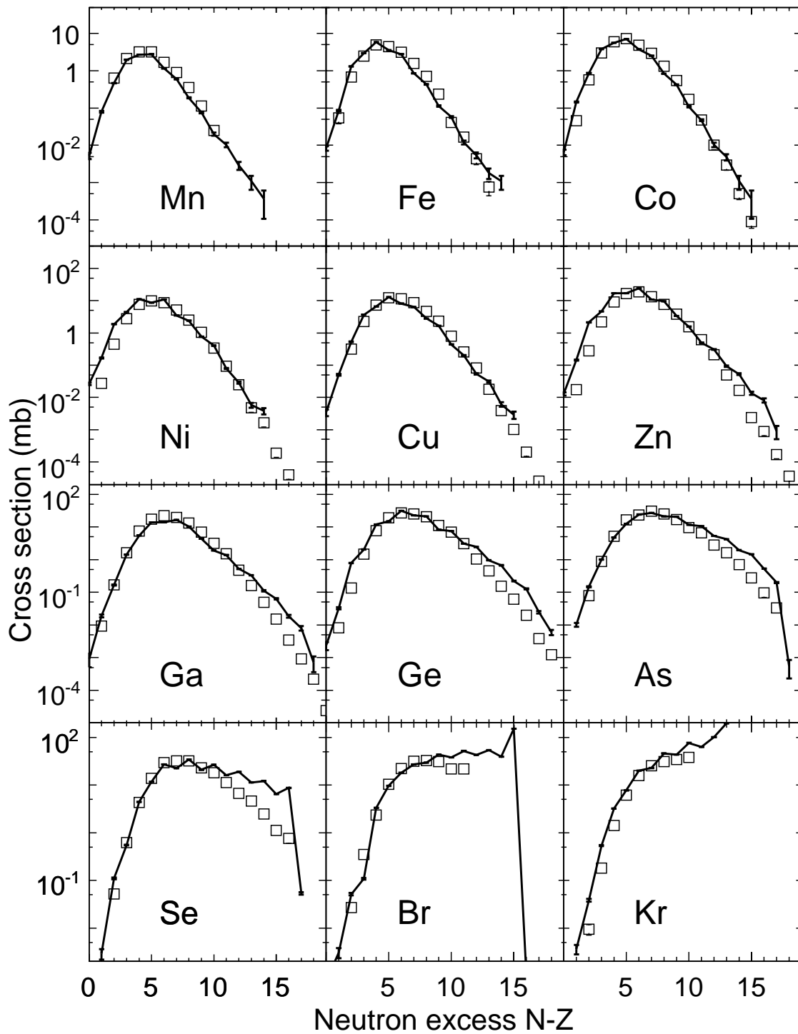
Figure 18: Measured cross sections for ^{86}\text{Kr} fragmentation on ^9\text{Be} at 64 MeV/nucleon [50,51] compared with LAQGSM03.03 predictions.
