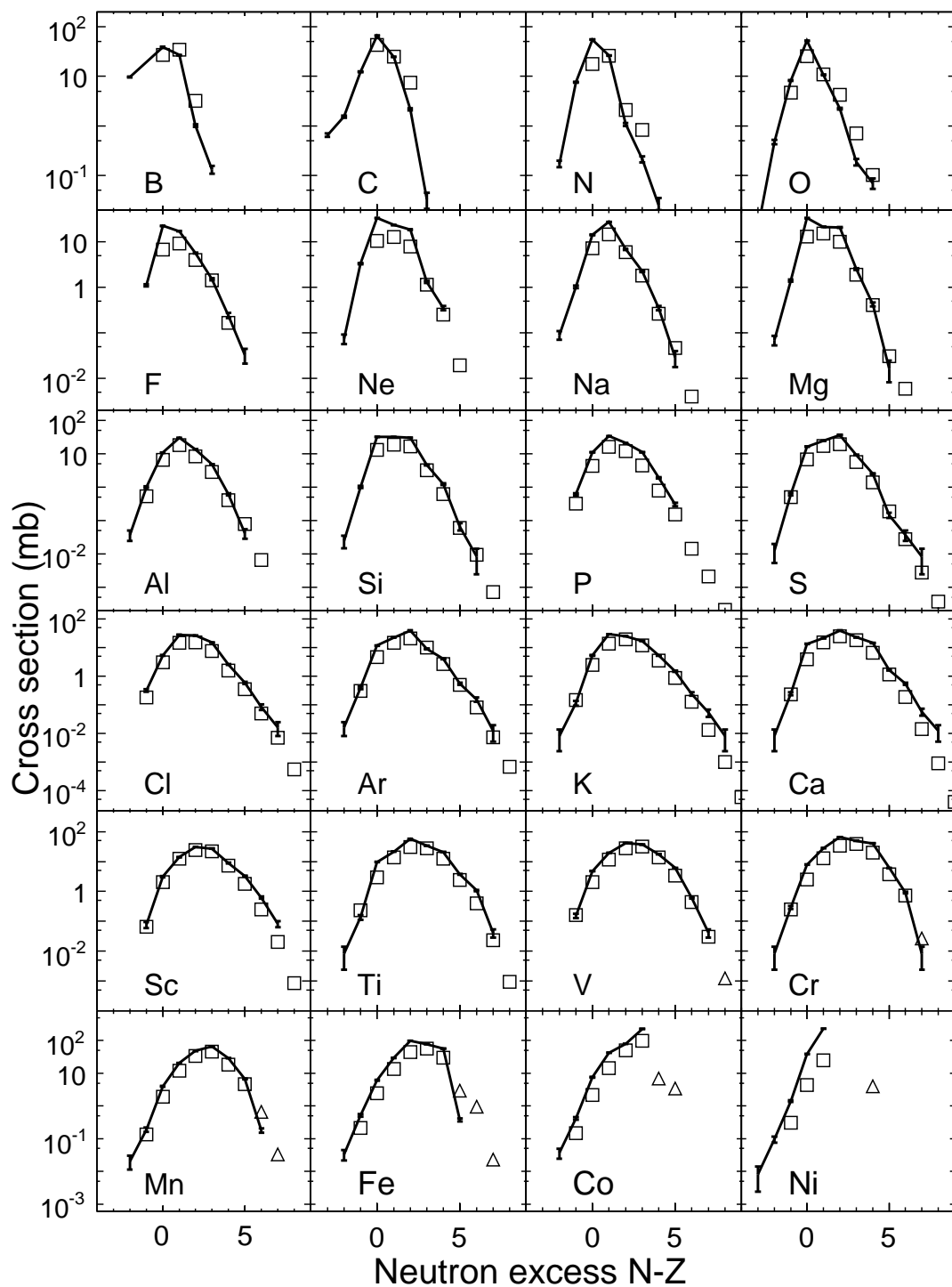
Figure 15: Measured cross sections for ^{58}\text{Ni} fragmentation on ^{181}\text{Ta} at 140 MeV/nucleon [49,50] compared with LAQGSM03.03 predictions.
