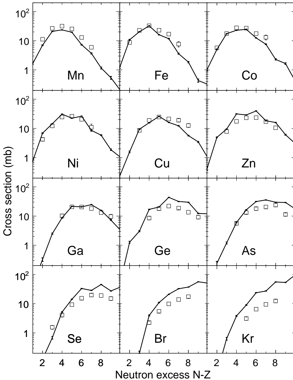
Figure 19: Measured cross sections for ^{86}\text{Kr} fragmentation on ^{181}\text{Ta} at 64 MeV/nucleon [50,51] compared with LAQGSM03.03 predictions.
