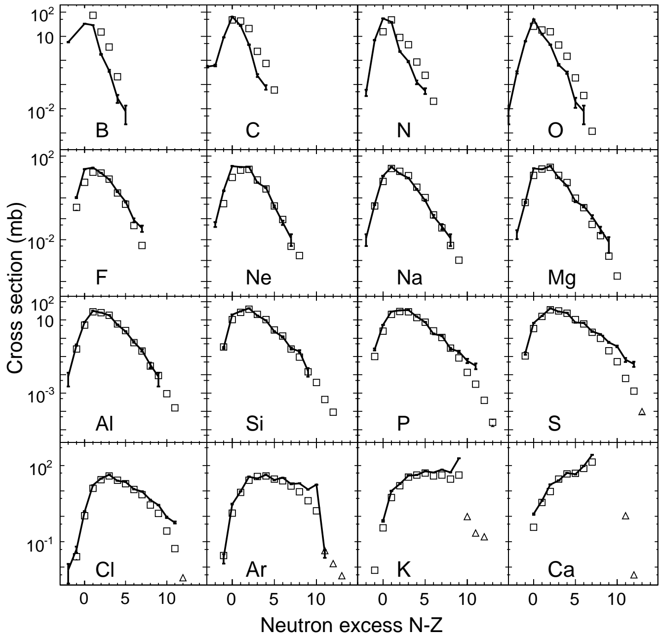
Figure 13: Measured cross sections for ^{48}\text{Ca} fragmentation on ^{181}\text{Ta} at 140 MeV/nucleon [49,50] compared with LAQGSM03.03 predictions.
