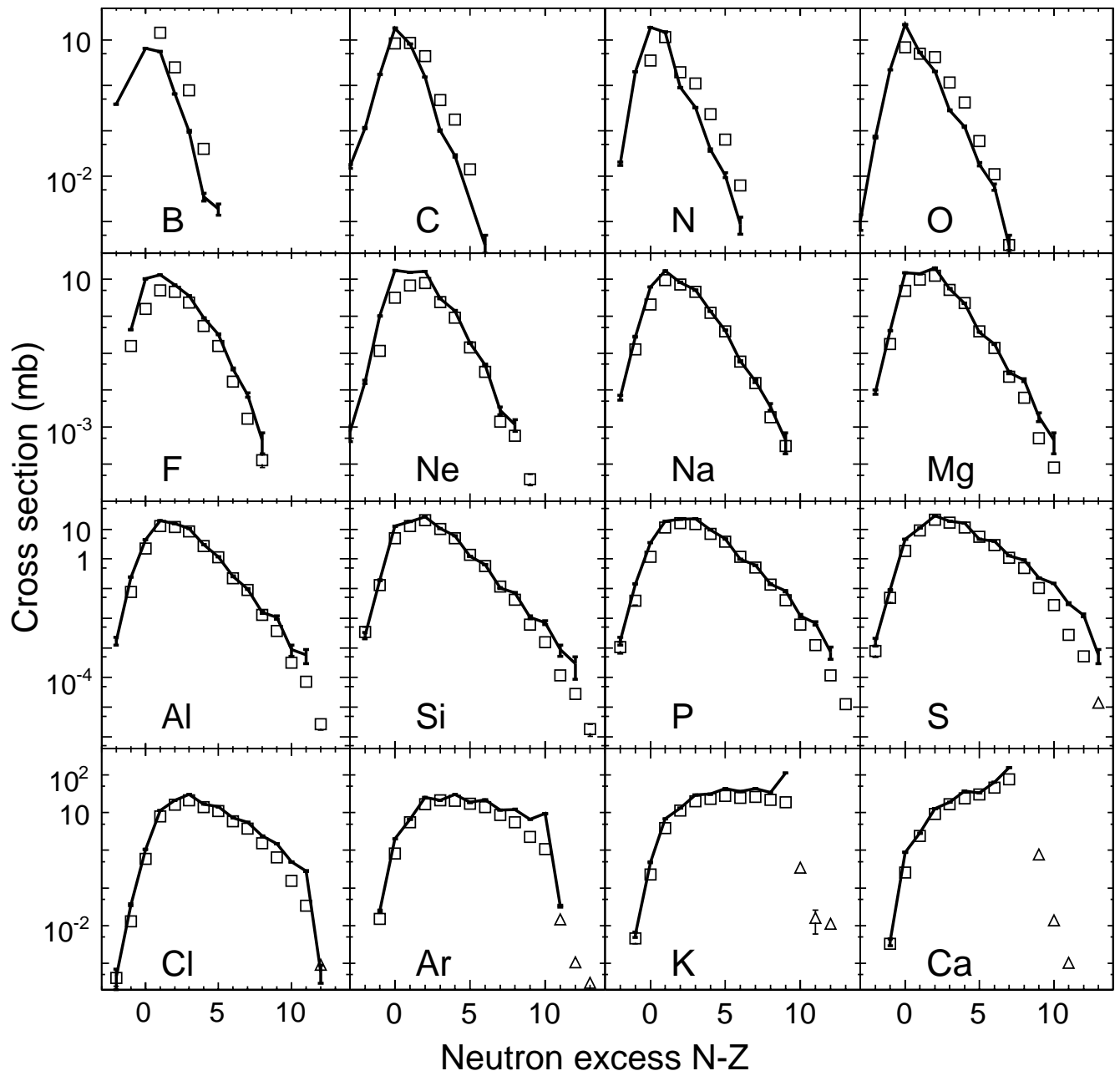
Figure 12: Measured cross sections for ^{48}\text{Ca} fragmentation on ^9\text{Be} at 140 MeV/nucleon [49,50] compared with LAQGSM03.03 predictions.
