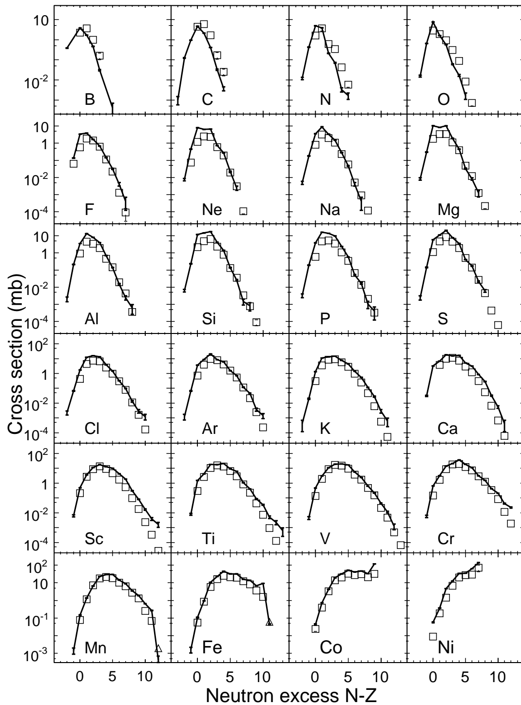
Figure 16: Measured cross sections for ^{64}\text{Ni} fragmentation on ^9\text{Be} at 140 MeV/nucleon [49,50] compared with LAQGSM03.03 predictions.
