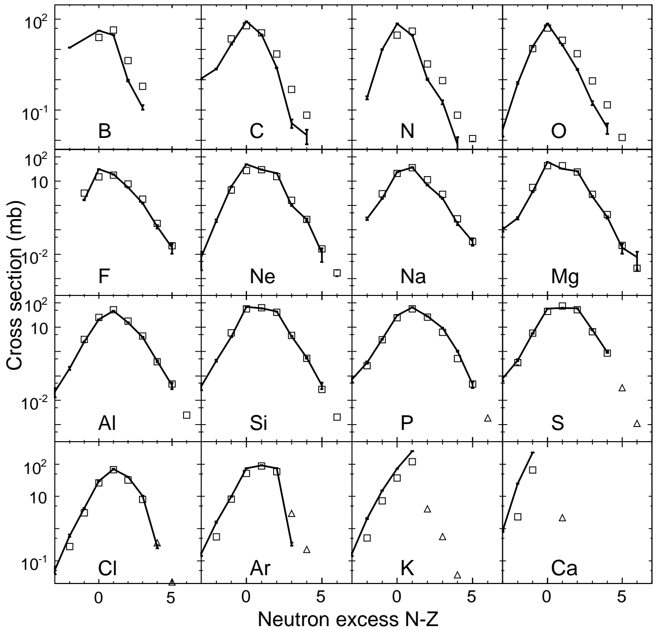
Figure 11: Measured cross sections for 40 Ca fragmentation on 181 Ta at 140 MeV/nucleon [49,50] compared with LAQGSM03.03 predictions.
