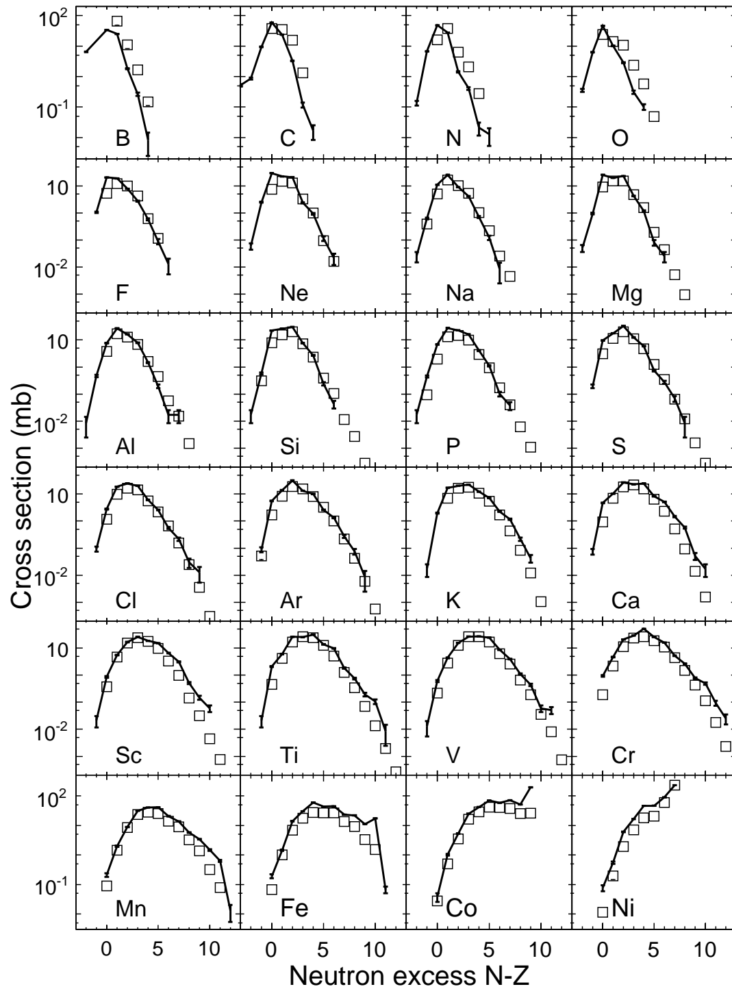
Figure 17: Measured cross sections for ^{64}\text{Ni} fragmentation on ^{181}\text{Ta} at 140 MeV/nucleon [49,50] compared with LAQGSM03.03 predictions.
