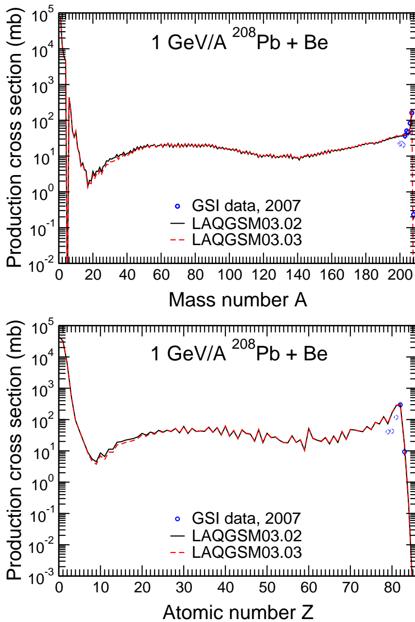
Figure 4: Mass- and charge-number distributions of the yield of all products from the reaction 1 GeV/nucleon ^{208}\text{Pb} + ^9\text{Be} . Symbols are GSI measurements of Nieto et al. [38]; dashed lines are results from LAQGSM03.03, while solid lines are results from LAQGSM03.02 [12].
