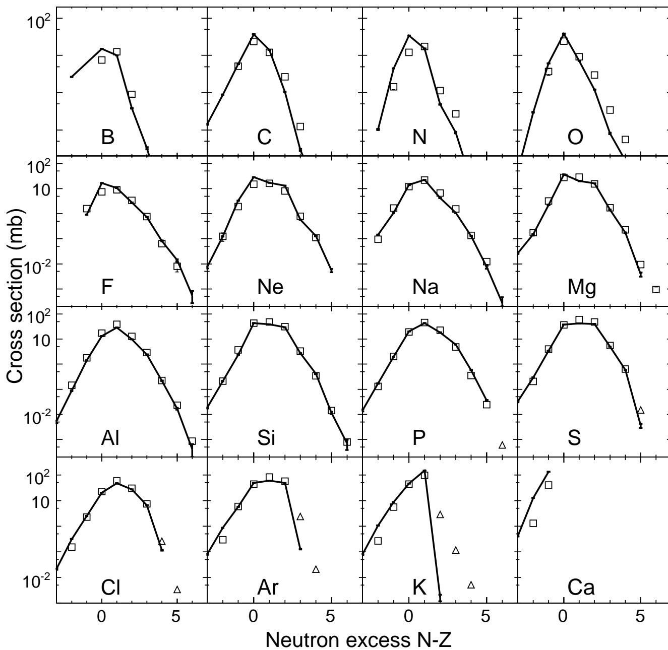
Figure 10: Measured cross sections for 40 Ca fragmentation on 9 Be at 140 MeV/nucleon [49,50] compared with LAQGSM03.03 predictions.
