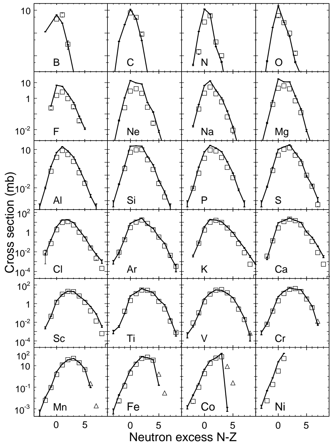
Figure 14: Measured cross sections for ^{58}\text{Ni} fragmentation on ^9\text{Be} at 140 MeV/nucleon [49,50] compared with LAQGSM03.03 predictions.
