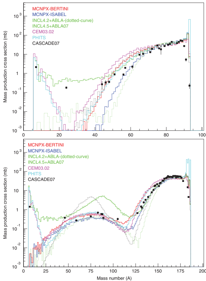
FIG. 3. (Color online) Calculated mass distributions of product yields for the targets of ^{93}\text{Nb} (top plot) and ^{\text{nat}}\text{W} (bottom plot) irradiated with 0.8-GeV protons compared with the measured cumulative and supracumulative yields.
