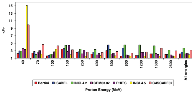
FIG. 7. (Color online) The same as in Fig. 4, but for ^{93}\text{Nb} .
