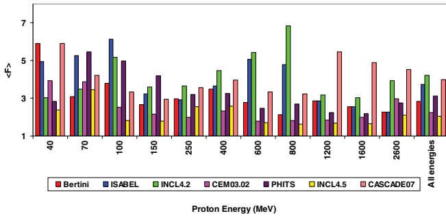
FIG. 5. (Color online) The same as in Fig. 4, but for ^{56}\text{Fe} .
