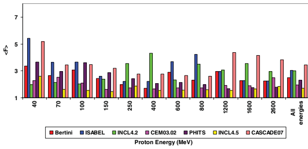
FIG. 6. (Color online) The same as in Fig. 4, but for ^{\text{nat}}\text{Ni} .
