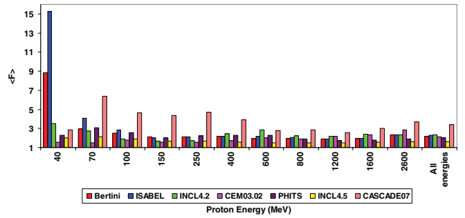
FIG. 10. (Color online) The same as in Fig. 4, but for ^{\text{nat}}\text{Pb} .
