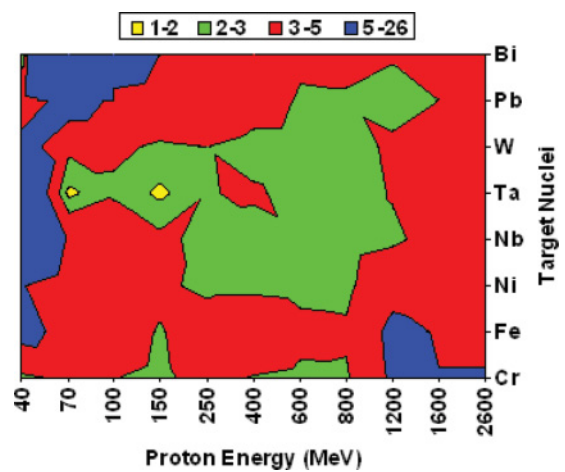
FIG. 18. (Color online) The same as in Fig. 12, but for the CASCADE07 code.
