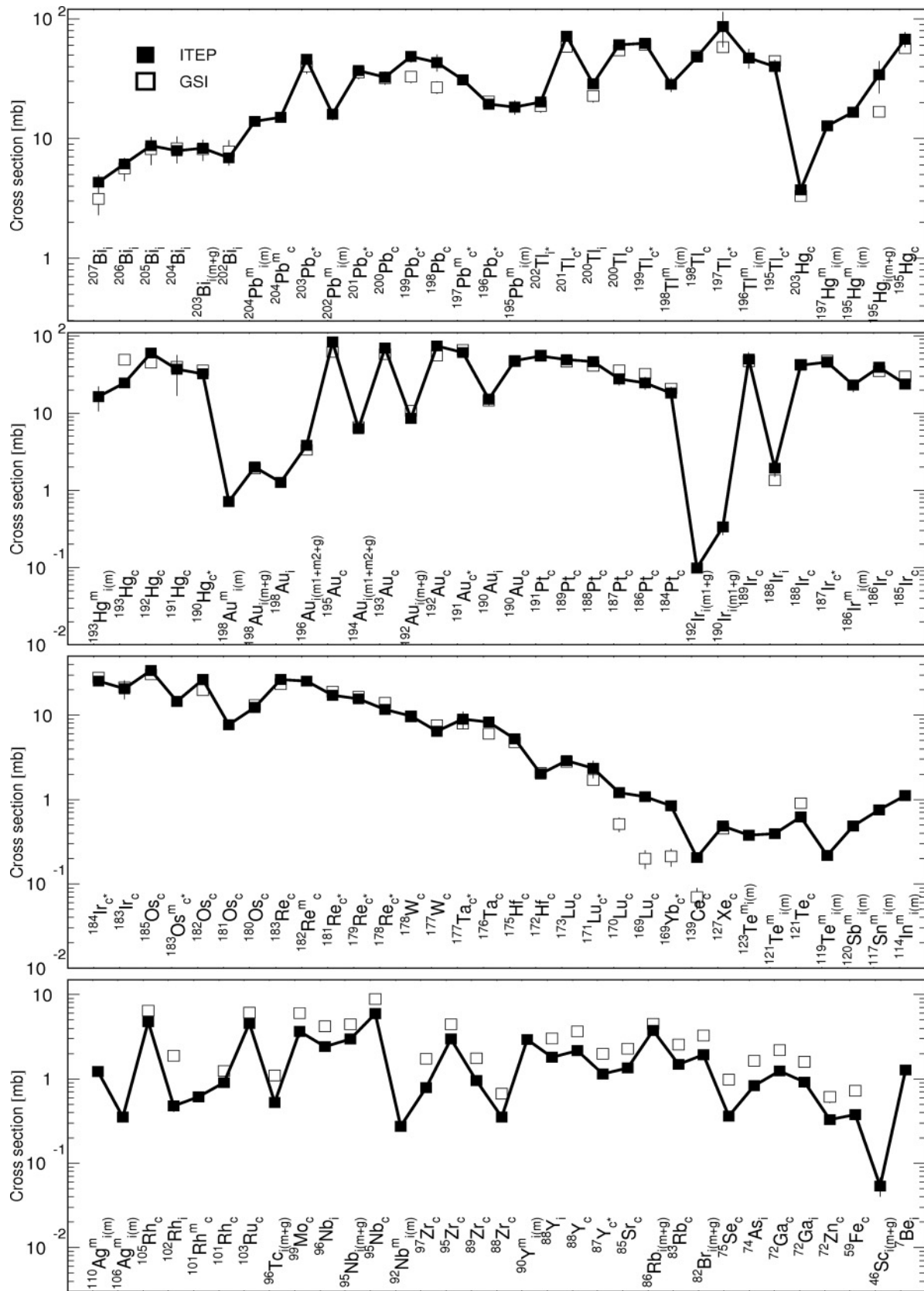
FIG. 19. Comparison of the nuclides production cross sections measured by the activation method at ITEP with estimated here cumulative yields from the independent cross sections by the inverse kinematics method measured at GSI for a ^{208}\text{Pb} target irradiated with 500-MeV protons.
