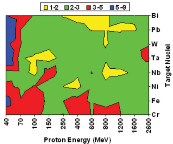
FIG. 12. (Color online) Predictive accuracy of the BERTINI code for various proton energies and target masses.
