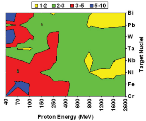
FIG. 17. (Color online) The same as in Fig. 12, but for the PHITS code.
