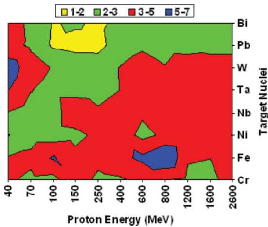
FIG. 15. (Color online) The same as in Fig. 12, but for the INCL4.2 + ABLA code.
