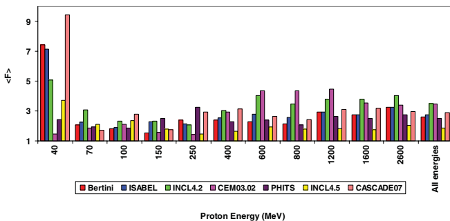
FIG. 8. (Color online) The same as in Fig. 4, but for ^{181}\text{Ta} .
